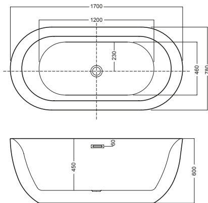
vasca 170x78 BT_01 bathtub 170x78 BT_01
