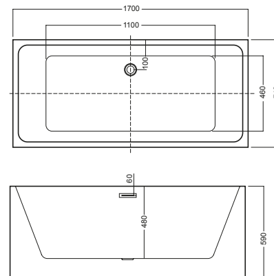
vasca 170x74 BT_02 bathtub 170x74 BT_02
