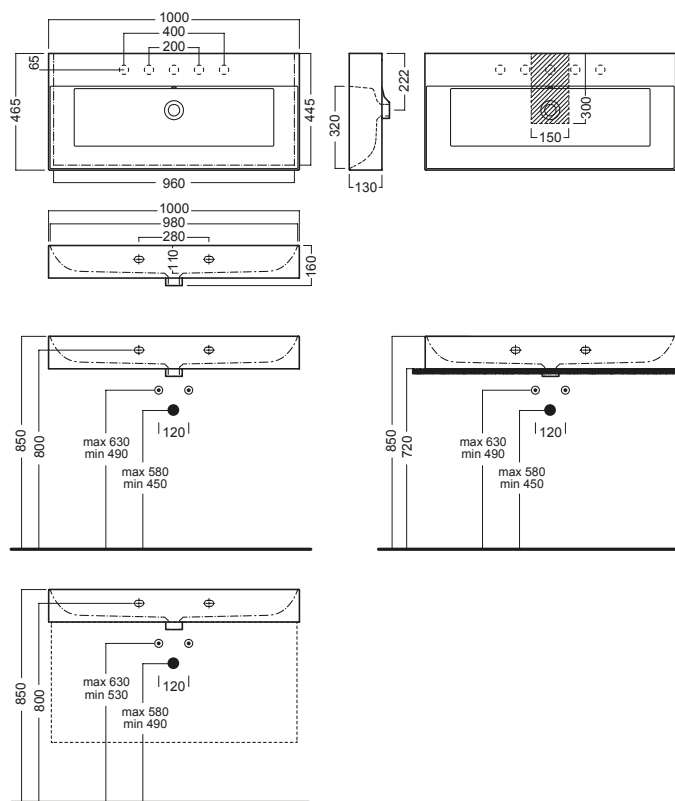
lavabo 100x46,5 washbasin 100x46,5
