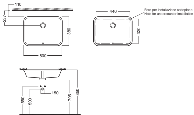
lavabo 50x38 washbasin 50x38
